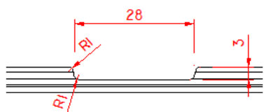
Type 50 (28 x 3 mm) 4 layers of veneer
